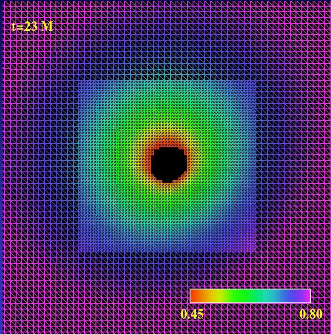
Lapse \alpha , z=0 slice, NOTE change of color scale
