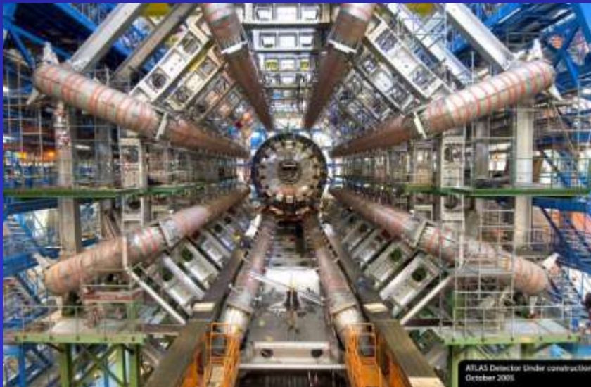
ATLAS experiment at the LHC
