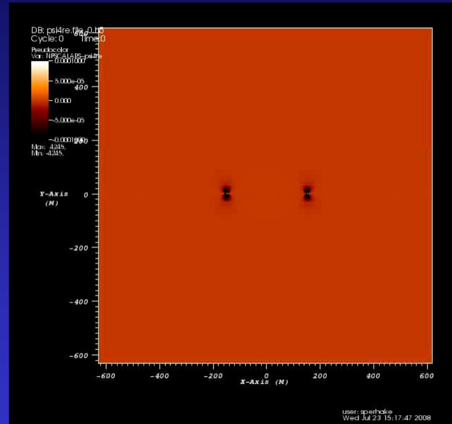
\gamma=1.5 grazing collision
