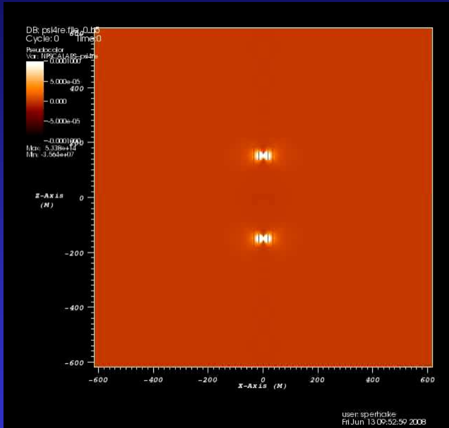
\gamma=2.9 head on collision
