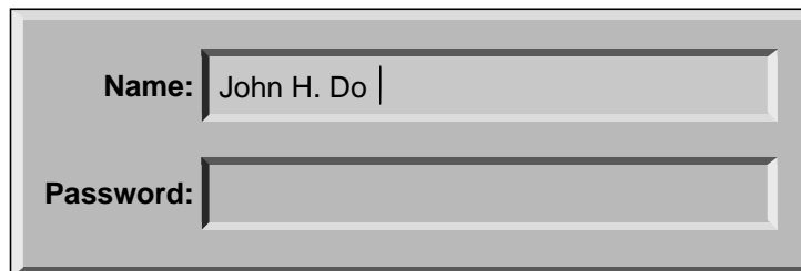
Figure 3.3: Input fields
