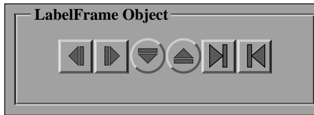
Figure 15.1: Labelframe Classes
