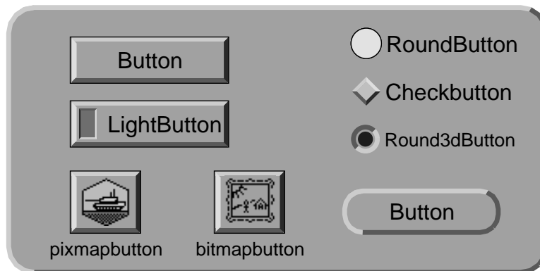
Figure 16.1: Button Classes
