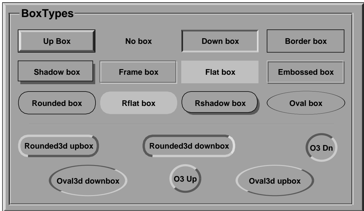
Figure 3.1: All boxtypes
