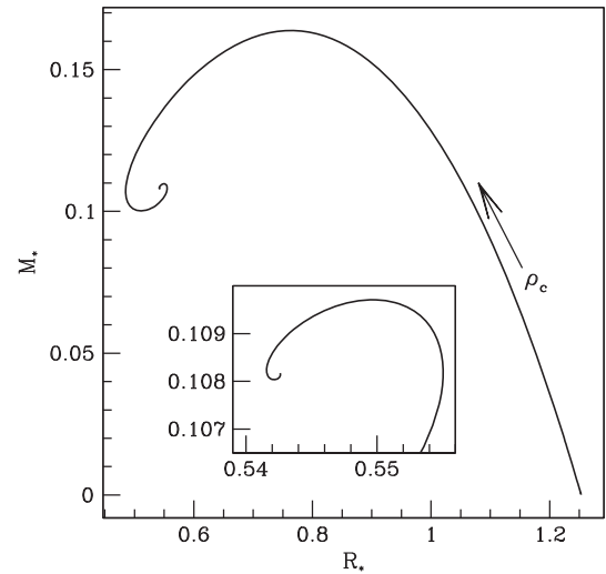
FIG. 1. Mass versus radius of TOV solutions using \Gamma = 2 and K = 1 with the polytropic EOS (37). In the inset, we show a detailed view of the spiraling behavior. The arrow along the right side of the curve indicates the direction of increasing central density.
