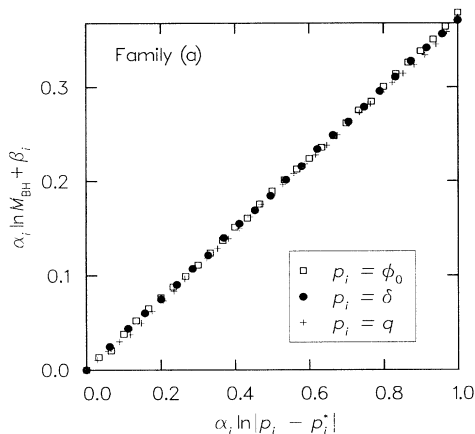
FIG. 4. Illustration of the conjectured mass-scaling relation (12). Data from three separate one-parameter variations of the pulse shape shown in Fig. 1(a) are shown. For each variation, I chose constants \alpha_i and \beta_i to normalize the ranges of the abscissa and place the data point corresponding to the smallest black hole in each family at the origin. The maximum ordinate value is 1/e .
