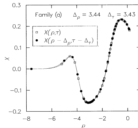
FIG. 2. Illustration of the rescaling or echoing property observed in near-critical evolution of the scalar field. The curve marked with open squares shows the profile of the scalar field variable, X , at some proper central time T_0 . The curve marked with solid circles is the profile at a later time T_0 + e^{\Delta\tau} but on a scale e^{\Delta\rho} \approx 30 times smaller.
