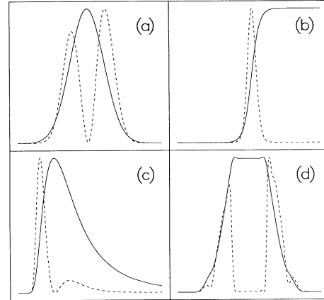
FIG. 1. Typical initial profiles of the scalar field \phi (solid lines) and the radial mass-energy density dm/dr (dotted lines) for the four families defined in Table I.
